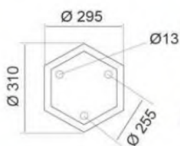
TRỤ 295 L850 x H4000 E27 x 3 16.450.000đ
