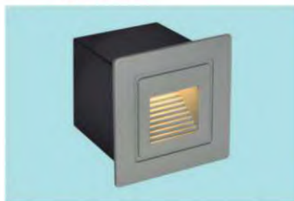
AT-19A COB 3W - IP54 □83 x W45 ⌀65 415.000đ
